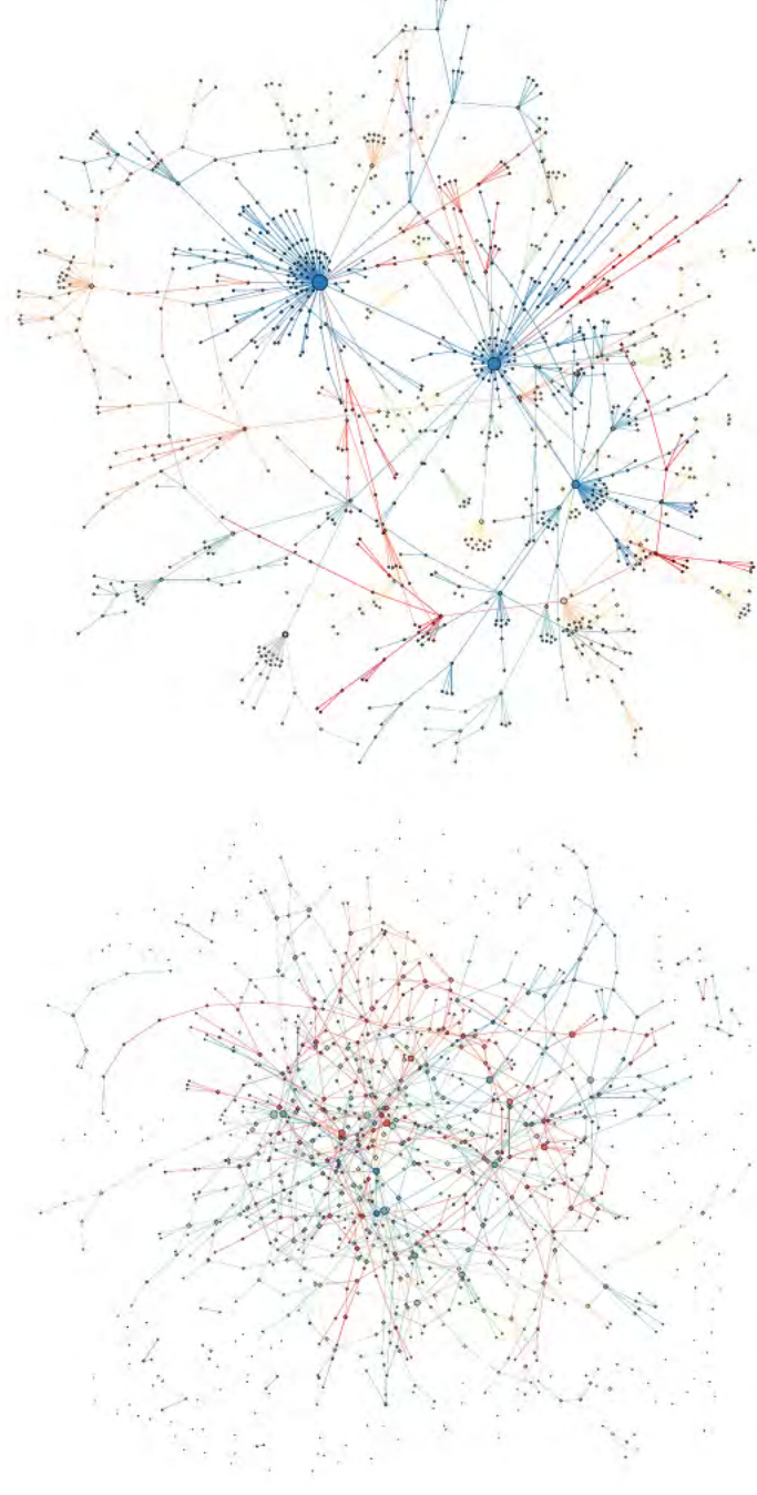
(a) E-R random network, average degree = 2. (b) BA scale-free network, average degree = 2. (c) BA scale-free network, average degree = 4.
